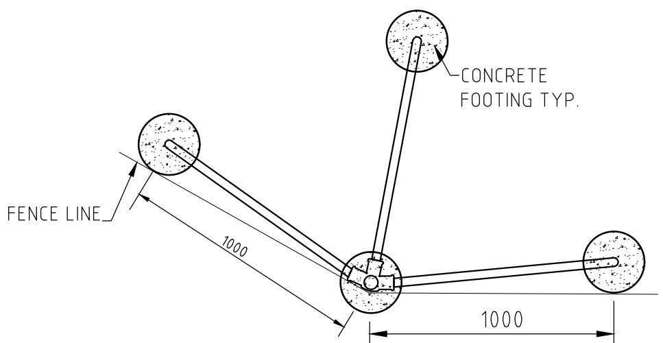
CORNER POST FOOTING PLAN(>90) SCALE 1:20
