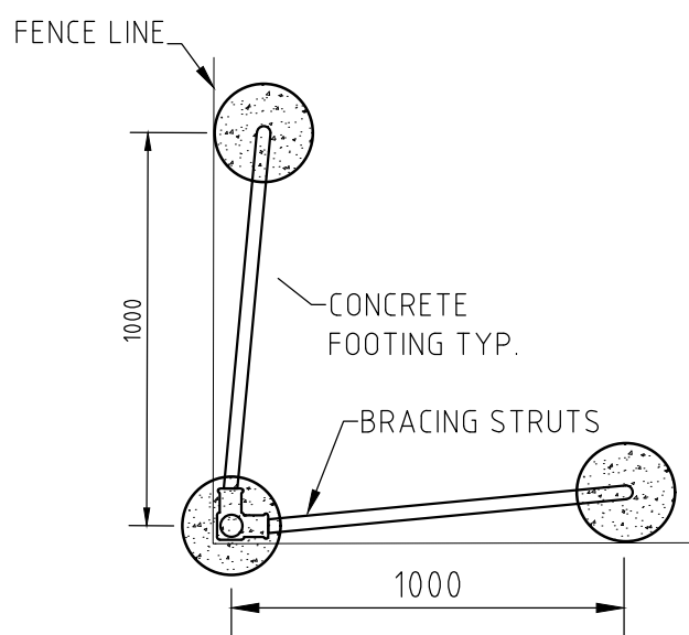
CORNER POST FOOTING PLAN(<90) SCALE 1:20
