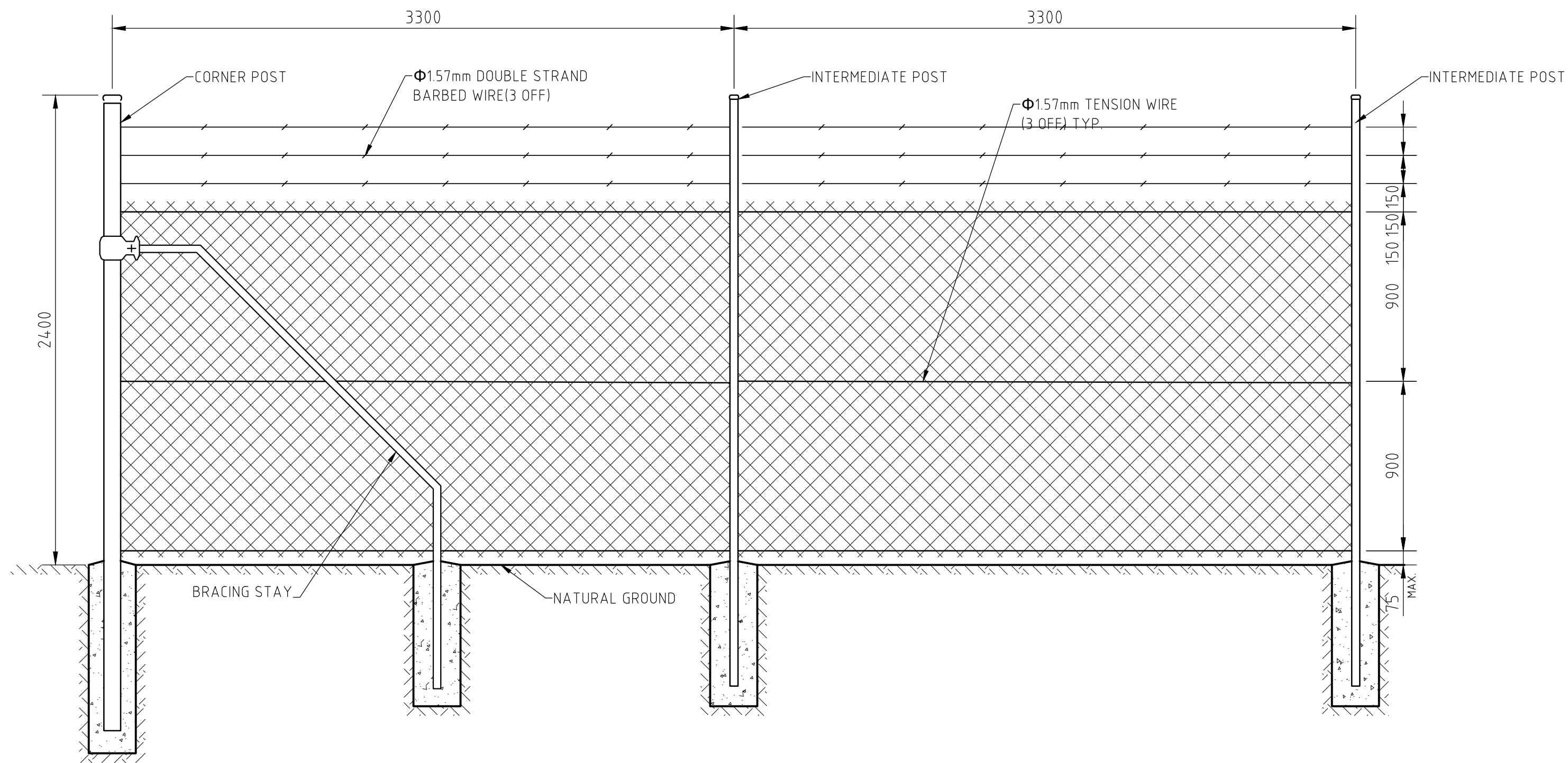
TYPICAL CHAIN MESH FENCE PANEL-3300 DISTANCE SCALE 1:20
