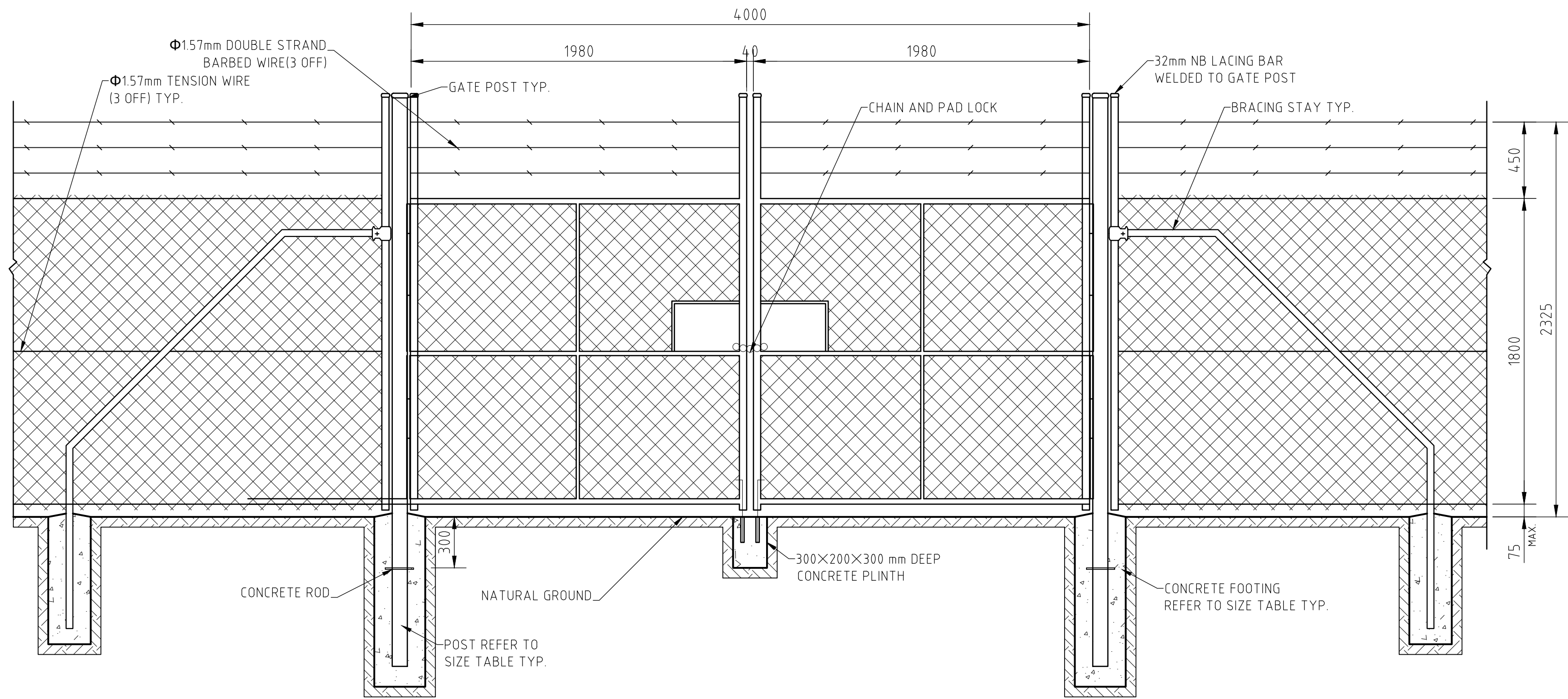
CHAIN LINK FABRIC FENCE AND OPENING DOUBLE GATE -4000 GATE SCALE 1:20
